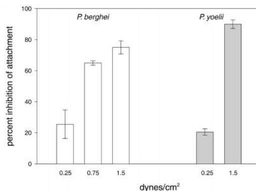
FIG. 2. Heparin inhibition of sporozoite attachment to HepG2 cells in a parallel plate flow chamber. Sporozoites were preincubated \pm 25 \mu\text{g/ml} of heparin for 15 min on ice, infused into the inlet tubing of the flow chamber, and then perfused over the cells at controlled flow rates. The wall shear stress was calculated as a function of flow rate. The perfusion time was inversely proportional to the flow rate so that for each point an equal number of sporozoites were allowed to perfuse over the cell monolayer. Nonadherent sporozoites were washed off with medium infused at 0.05 ml/min (resulting in a shear force of 0.25 dynes/cm 2 ) for 6 min. The cells were fixed, and sporozoites were stained as outlined previously. For each point, the entire area covered by the flow chamber was divided into 2, and \geq 100 fields per region were counted. Percent inhibition was calculated using the mean number of sporozoites attached in the absence of heparin with the same flow rate.
