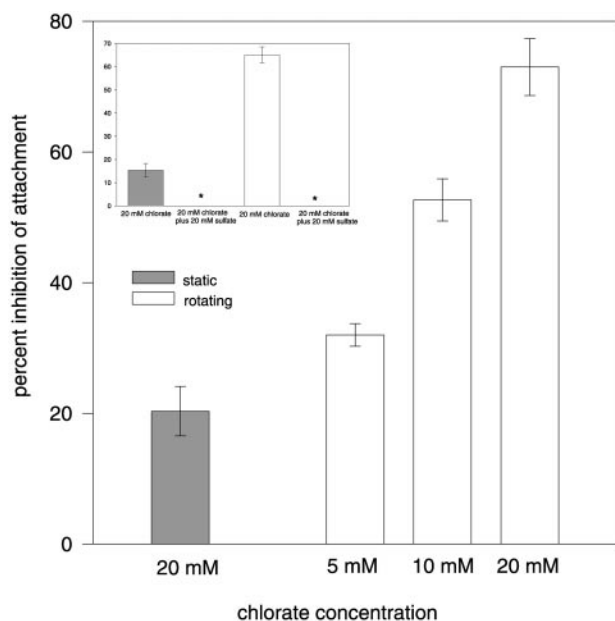
FIG. 7. Inhibition of sporozoite attachment to chlorate-treated HepG2 cells. HepG2 cells were plated in labtek chamber slides, and 2 days later the medium was replaced with low sulfate medium containing the indicated concentrations of chlorate. After 24 h, the chlorate-containing medium was removed, and P. berghei sporozoites in DMEM/FCS were added to each well. After 1 h at 37 °C under static (gray bars) or rotating conditions (white bars), unattached sporozoites were removed; the cells were fixed, and the attached sporozoites were stained. Shown is the percent inhibition of sporozoite attachment to cells in the presence of chlorate compared with the mean number of sporozoites attached in the absence of chlorate (under static or rotating conditions). Each point was plated in triplicate and shown are the means with standard deviations. Inset shows sporozoite attachment, under static and rotating conditions, to cells that had been incubated (as above) in medium with no chlorate, 20 mM chlorate, and 20 mM chlorate plus 20 mM magnesium sulfate. There was no inhibition of sporozoite attachment to cells in 20 mM chlorate plus 20 mM magnesium sulfate under both static and rotating conditions (asterisks indicate that the data were collected, but the error bar cannot be seen since it is 0). Each point was plated in triplicate and shown are the means with standard deviations.
