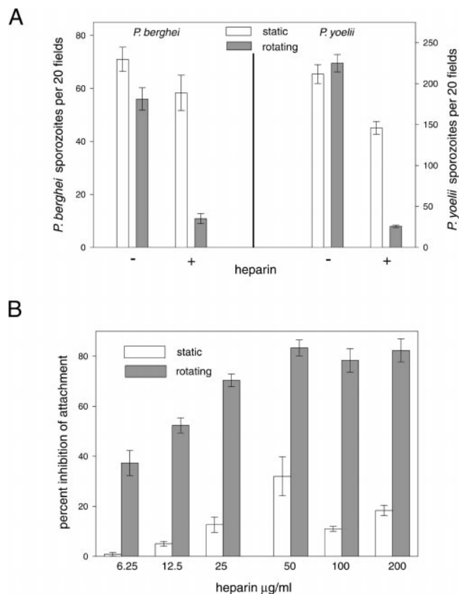
FIG. 1. Heparin is a better inhibitor of sporozoite attachment under conditions that mimic flow. Sporozoites were preincubated \pm 25 \mu\text{g/ml} of heparin (A) or the indicated concentration of heparin (B) for 15 min on ice and then plated on cells in the continued presence of heparin. After 1 h at 37 °C under static or rotating conditions, unattached sporozoites were removed by washing, and the attached sporozoites were visualized with the appropriate monoclonal antibody (mAb 3D11 for P. berghei and mAb NYS1 for P. yoelii ) and goat anti-mouse Ig conjugated to FITC. Each point was plated in triplicate and shown are the means with standard deviations. A, attachment of P. berghei and P. yoelii sporozoites to cells under static and rotating conditions. B, dose-dependent inhibition of P. berghei sporozoite attachment. Percent inhibition was calculated using the mean number of sporozoites attached in the absence of heparin under static or rotating conditions.
