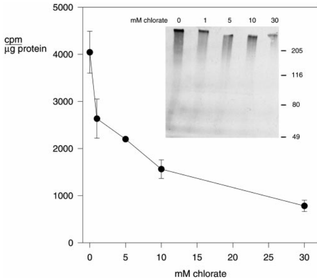
FIG. 5. Chlorate inhibits sulfate incorporation into proteoglycans of HepG2 cells. HepG2 cells were plated in 6-well plates in medium with the indicated concentration of chlorate. After 12 h, the medium was changed to low sulfate medium with the indicated concentrations of chlorate and [ ^{35} S]sodium sulfate. 12 h later the cells were washed, lysed, and total cell-associated counts/min were measured in a \beta -counter. Each point was performed in triplicate and shown as the means with standard deviations. Inset , lysates from chlorate-treated cells were loaded onto a 5% SDS-polyacrylamide gel that was then subjected to autoradiography. Equivalent amounts of protein were loaded onto each lane. Most of the labeled material migrated as a broad high molecular weight smear, typical of proteoglycans.
