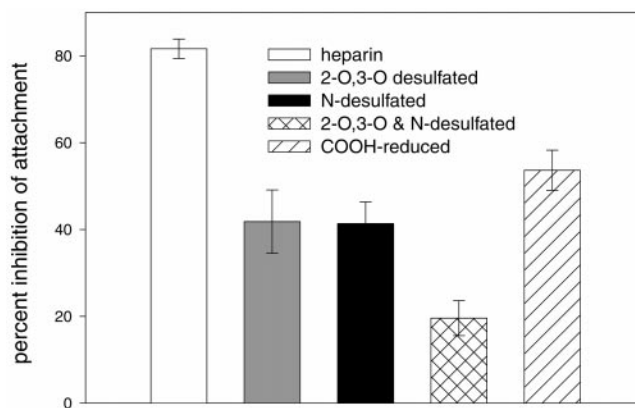
FIG. 8. Sporozoite attachment to HepG2 cells under rotating conditions in the presence of modified heparins. P. berghei sporozoites were preincubated for 15 min on ice in medium alone or with 25 µg/ml heparin (white bar), 2- O ,3- O -desulfated heparin (gray bar), N -desulfated heparin (black bar), 2- O ,3- O - and N -desulfated heparin (cross-hatched bar), and carboxy-reduced heparin (diagonally lined bar) and then added to HepG2 cells in labtek chamber slides. Sporozoite incubation with cells was under rotating conditions and in the continued presence of the inhibitor. After 1 h, unattached sporozoites were removed; the cells were fixed, and the attached sporozoites were stained and counted. Each point was plated in triplicate wells. Percent inhibition of sporozoite attachment was calculated using the mean number of sporozoites attached in the absence of heparin. This experiment was performed three times and shown are the pooled results from all three experiments.
