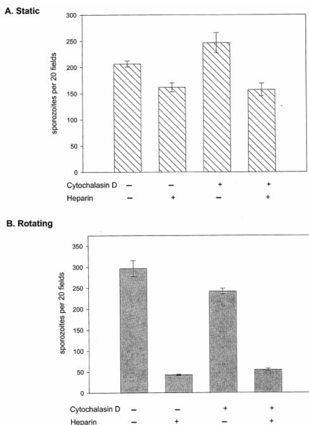
FIG. 3. Sporozoite attachment to HepG2 cells in the presence of heparin and cytochalasin D. P. berghei sporozoites were preincubated with or without 1 \mu M cytochalasin D \pm 25 \mu g/ml heparin and then plated on cells (in the continued presence of these compounds). After 1 h at 37 ^{\circ} C under static (A) or rotating (B) conditions, unattached sporozoites were removed, and the cells were stained with a double-staining procedure that allows the differentiation of intracellular from extracellular sporozoites. Each point was plated in triplicate and shown are the means with standard deviations of the total number of sporozoites attached to the cells. Invasion data for this experiment is not shown; however, in the presence of cytochalasin D there was no invasion, and in the absence of cytochalasin D, \sim 40% of attached sporozoites were found intracellularly regardless of whether heparin was present or not.
