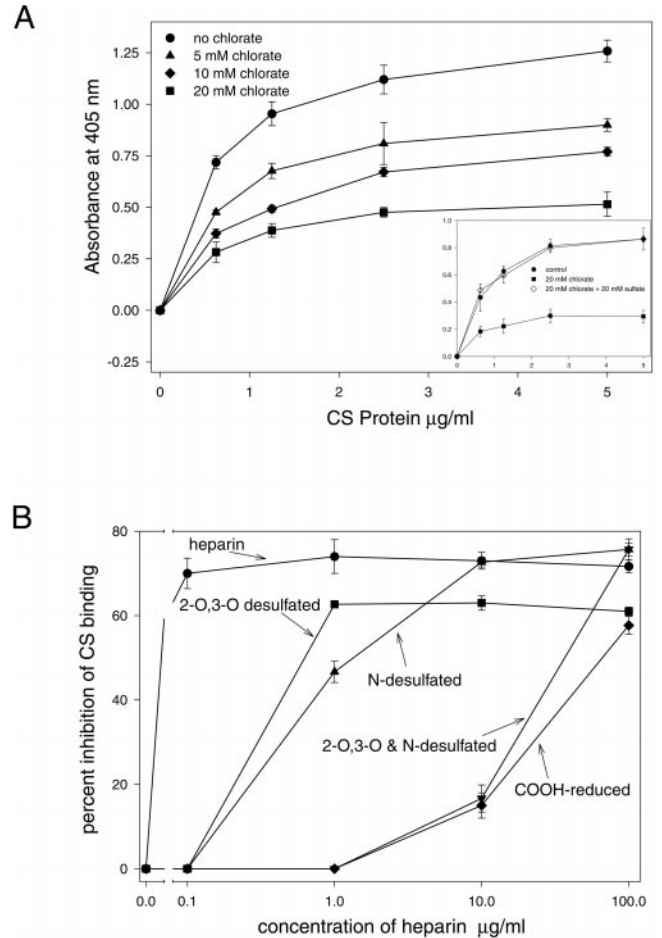
FIG. 6. A, CS binding to chlorate-treated HepG2 cells. Cells were plated in 96-well plates and grown in low sulfate medium with the indicated concentrations of chlorate. After 18–24 h, they were fixed, blocked, and incubated with increasing amounts of CS protein. CS binding was revealed with mAb 2A10 specific for the CS repeats, followed by anti-mouse Ig conjugated to horseradish peroxidase and peroxidase substrate. The CS binding curves for cells grown in 20 mM chlorate (squares), 10 mM chlorate (diamonds), 5 mM chlorate (triangles), and no added chlorate (circles) are shown. Each point was assayed in triplicate, and the means with standard deviations are shown. Inset shows CS binding curves for a control experiment where cells were grown in low sulfate medium with 20 mM chlorate (squares), 20 mM chlorate plus 20 mM magnesium sulfate (open diamonds), or no chlorate (circles). B, inhibition of CS binding to HepG2 cells with modified heparins. 5 \mu g/ml CS was preincubated with the indicated concentrations of each heparin for 30 min at 37 ^{\circ} C. These solutions were then added to paraformaldehyde-fixed HepG2 cells for 1 h at 37 ^{\circ} C; the cells were washed, and bound CS was determined using iodinated mAb 2A10, specific for the CS repeats. Shown is the percent inhibition of binding of CS to HepG2 cells in the presence of inhibitor compared with results obtained in the absence of inhibitor. Inhibitors were heparin (circles), 2-O,3-O-desulfated heparin (squares), N-desulfated heparin (triangles), 2-O,3-O- and N-desulfated heparin (inverted triangles), and carboxy-reduced heparin (diamonds). Each inhibitor concentration was assayed in triplicate, and the means with standard deviations are shown.
